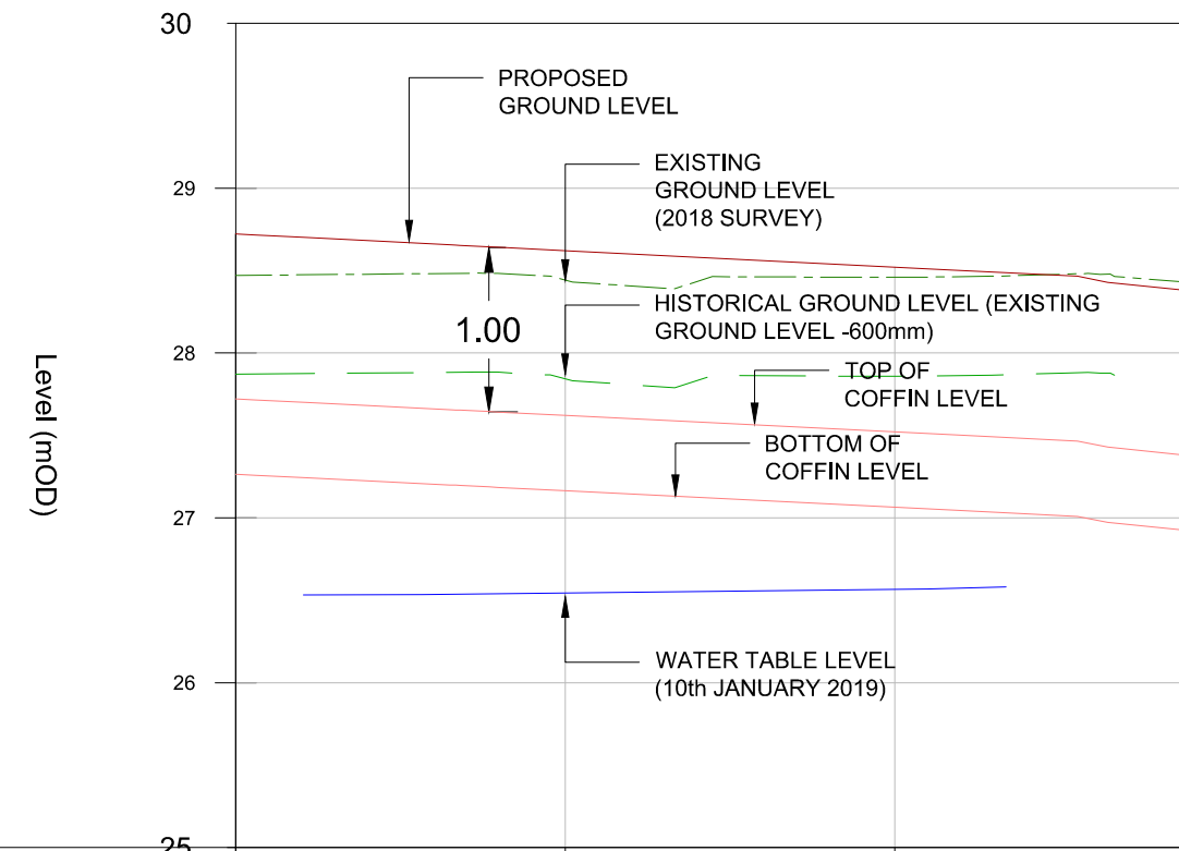
SECTION E-E - LONGSECTION SCALE: H 1:250,V 1:50. DATUM: 25.000
